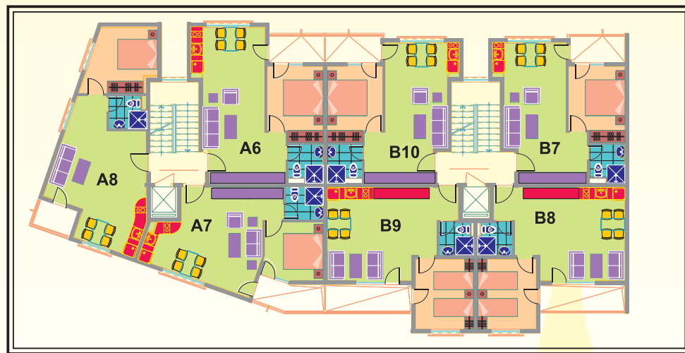
Block 1- floor 1
